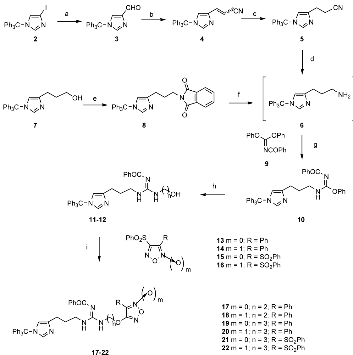
Scheme 1. (a) EtMgBr, DMF, rt; (b) NaNH_2 , (EtO)_2P(O)CH_2CN , THF, reflux; (c) H_2 , Pd/C, THF; (d) LiAlH_4/AlCl_3 , Et_2O/THF/(2:1) , rt; (e) PPh_3 , Phthalimide, DIAD, THF, 0 °C; (f) 40% aq CH_3NH_2 , EtOH, rt; (g) 9 , CH_2Cl_2 ; (h) 2-aminoethanol or 3-aminopropan-1-ol, THF, reflux; (i) 50% aq NaOH, 20–25 °C.
